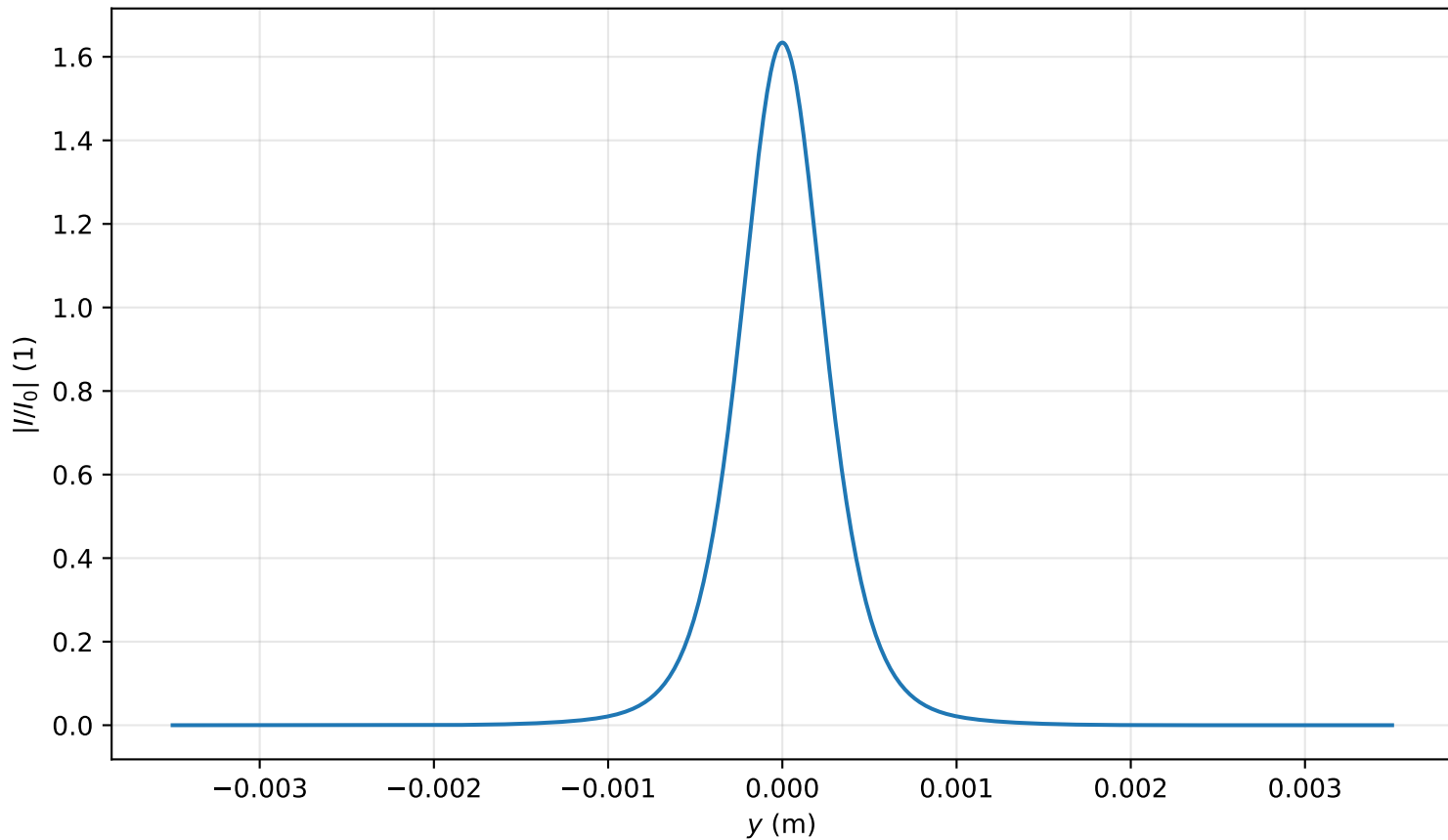
Intensity profile I(x=0, y, z=2.070)/I_0 , P_{in}=0.9P_{cr} , artificial time
